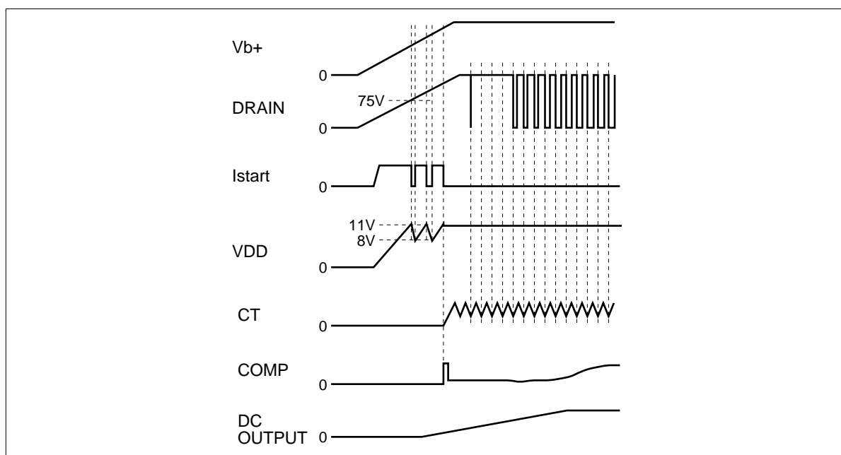
Figure 1 Start-Up Timing
