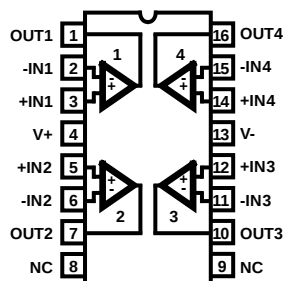
HA5104/5114 (SOIC) TOP VIEW
