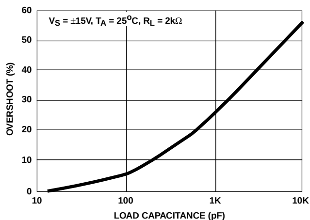
FIGURE 25. SMALL SIGNAL OVERSHOOT vs C_{LOAD}
