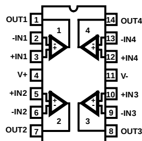
HA-5104/5114 (PDIP, CERDIP) TOP VIEW
