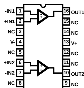
HA-5102/5112 (SOIC) TOP VIEW
