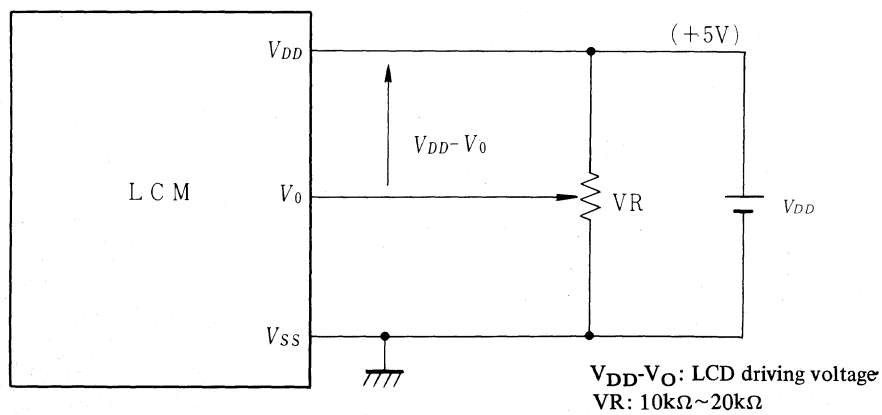
Fig. 4 Power supply
