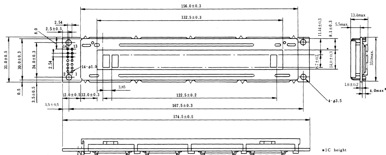
Fig. 2 External dimensions
