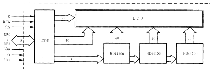
Fig. 3 Block diagram
