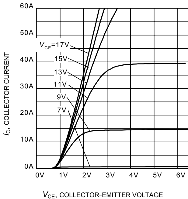
Figure 5. Typical output characteristic ( T_J = 25^\circ C )
