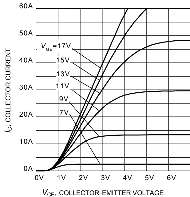
Figure 6. Typical output characteristic ( T_J = 150^\circ C )
