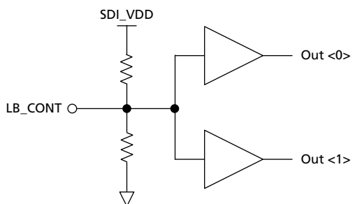
Figure 3-6: LB_CONT
