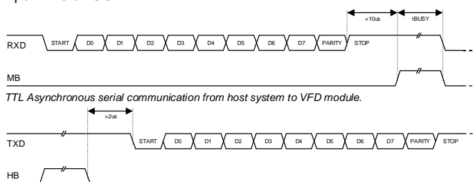
TTL Asynchronous serial communication from VFD module to host system.
