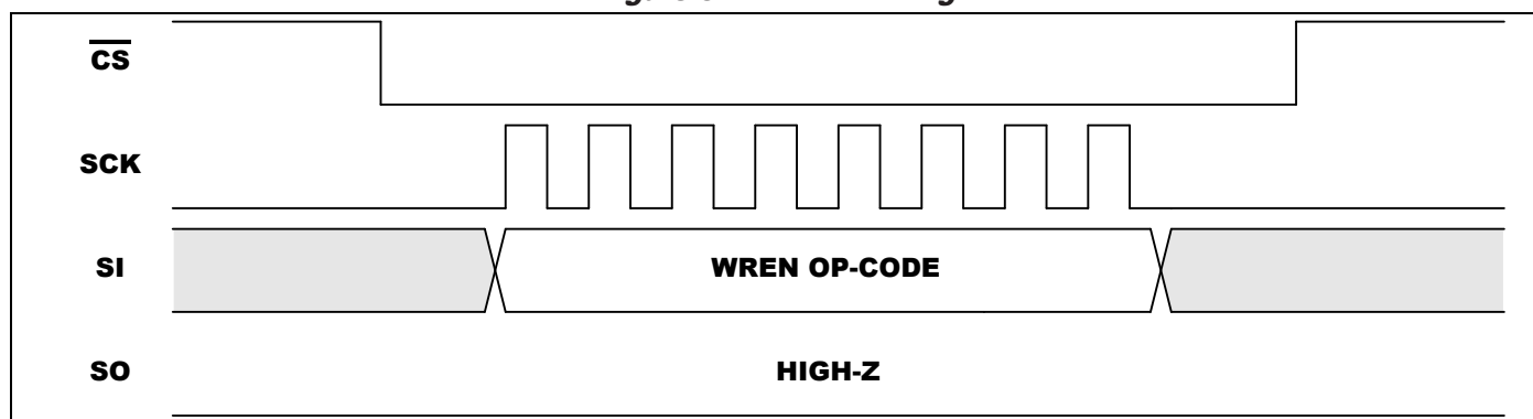
Figure 5-2. WREN Timing
