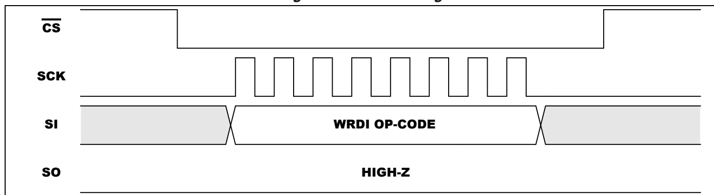
Figure 5-3. WRDI Timing
