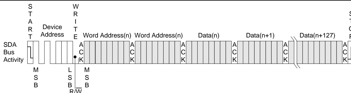
Figure 5-7. Page Write
