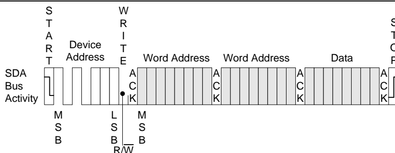
Figure 5-6. Byte Write
