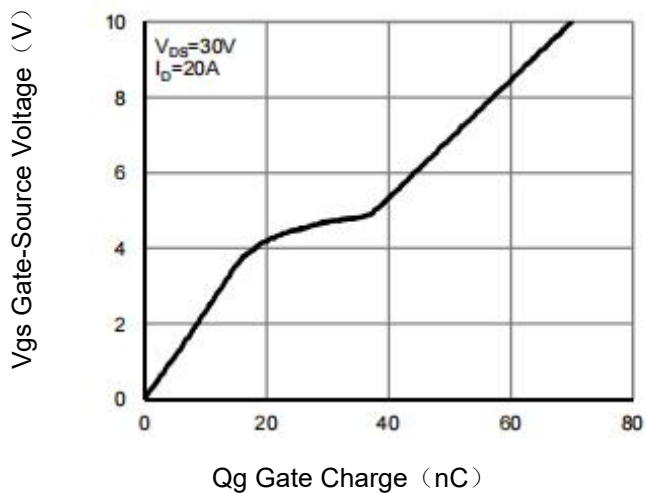
Figure 3. Gate Charge
