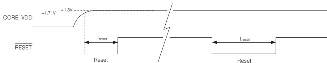
Figure 3-23: Reset pulse
