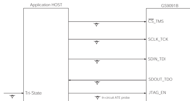
Figure 3-22: System JTAG
