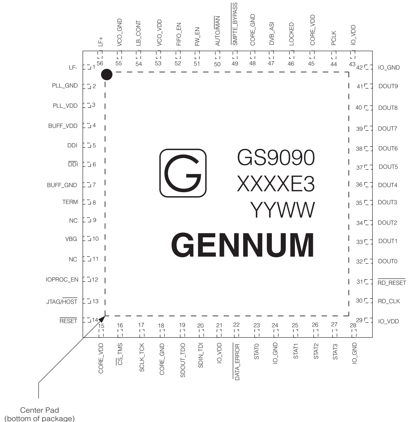
Figure 1-1: Pin Assignment
