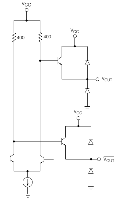
Fig. 2 Output Circuit (Pins 3, 4 and 5, 6)
