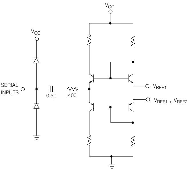
Fig. 1 Input Circuit (Pins 11 and 12)
