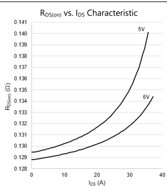
Figure 4: R_{DS(on)} vs. I_{DS} at T_J = 150^\circ\text{C}
