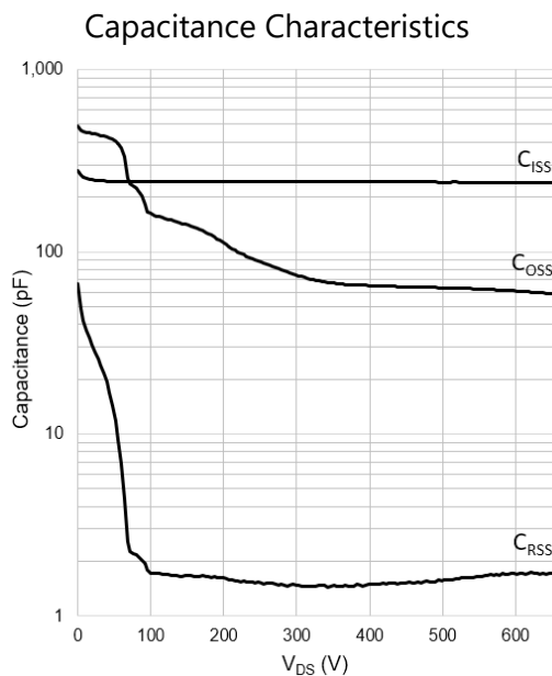
Figure 7: Typical C_{ISS} , C_{OSS} , C_{RSS} vs. V_{DS}
