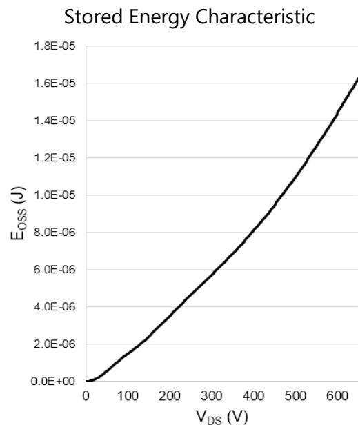
Figure 8: Typical C_{OSS} Stored Energy
