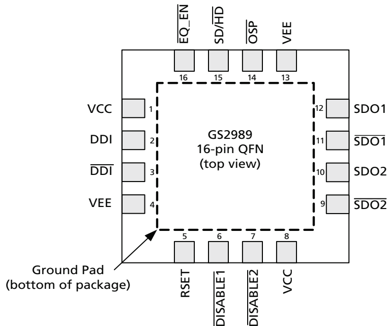
Figure 1-1: 16-Pin QFN
