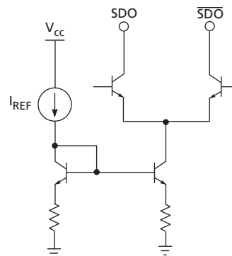
Figure 3-2: Differential Output Stage (SDO1/SDO1-bar, SDO2/SDO2-bar)
