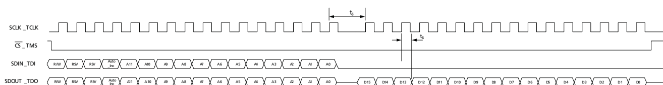
Figure 4-43: Read Mode
