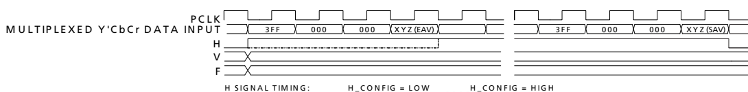
Figure 4-11: H:V:F Output Timing - SD 10-bit Output Mode
