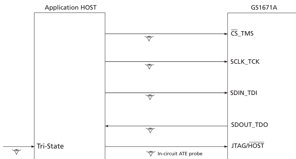
Figure 4-46: System JTAG
