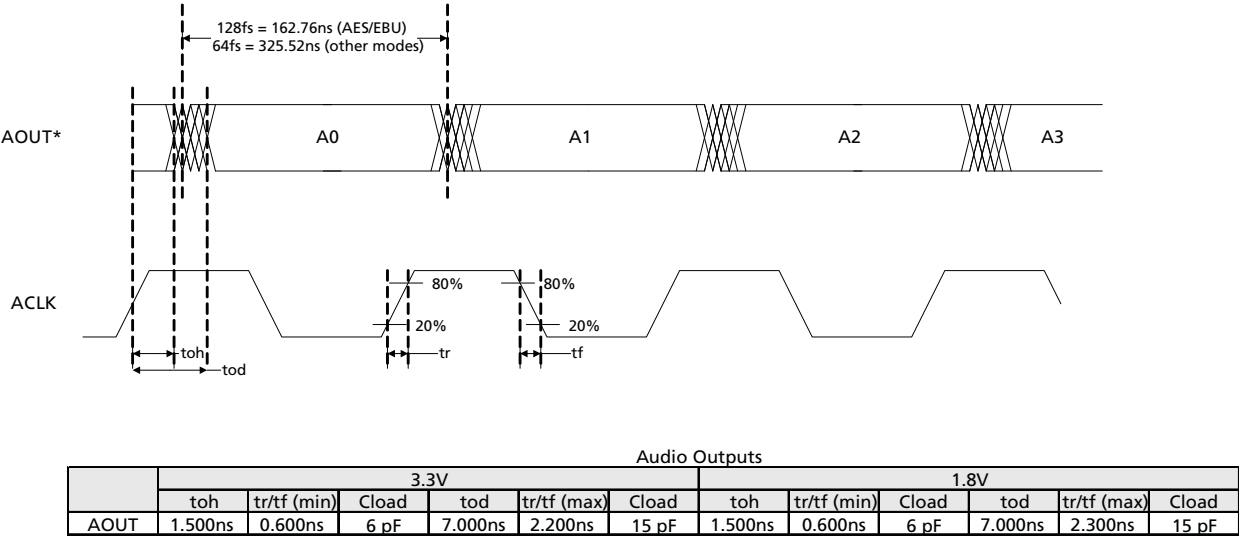
Figure 4-27: ACLK to Data Signal Output Timing
