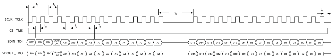
Figure 4-42: Write Mode
