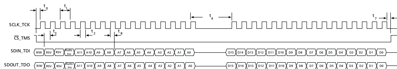
Figure 4-19: Write Mode
