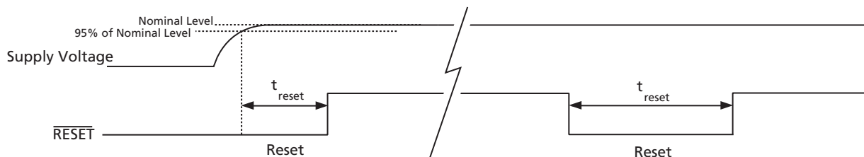
Figure 4-22: Reset Pulse
