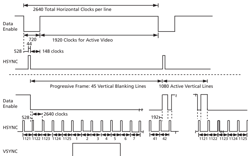
Figure 4-12: H:V:DE Input Timing 1920 x 1080p @ 23.94/24 (Format 32)
