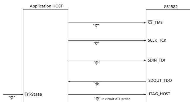
Figure 4-32: System JTAG
