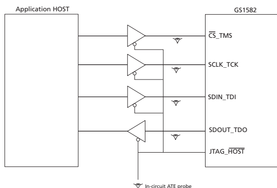
Figure 4-31: In-Circuit JTAG
