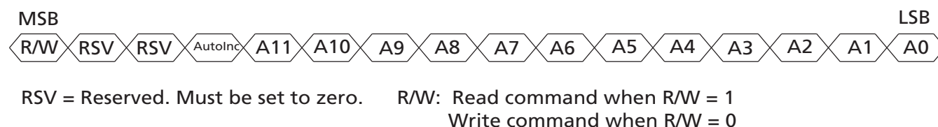
Figure 4-27: Command Word
