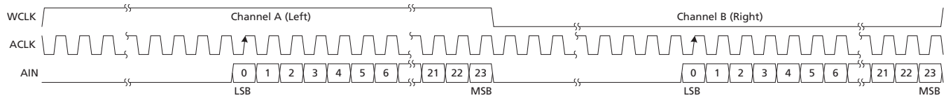
Figure 4-24: Serial Audio Input: Right Justified; LSB First
