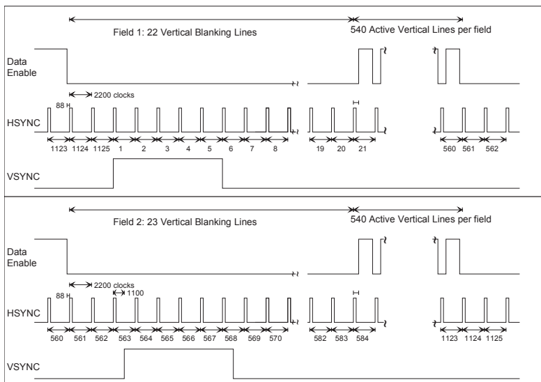
Figure 4-4: HSYNC:VSYNC:DE Input Timing 1920 x 1080i @ 59.94/60
