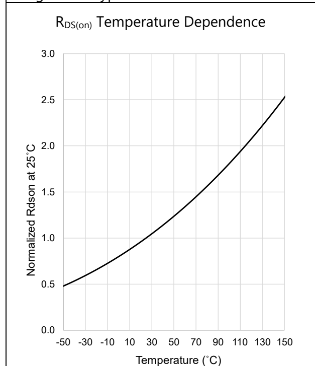
Figure 12: Normalized R_{DS(on)} as a function of T_J
