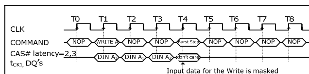
Termination of a Burst Write Operation (Burst Length = X, CAS# Latency = 2, 3)
