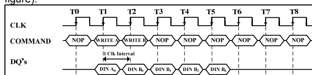
Write Interrupted by a Write (Burst Length = 4, CAS# Latency = 2, 3)
