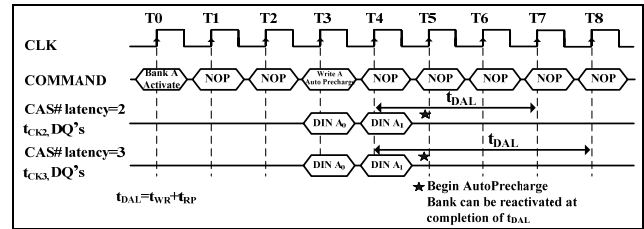
Burst Write with Auto-Precharge (Burst Length = 2, CAS# Latency = 2, 3)
