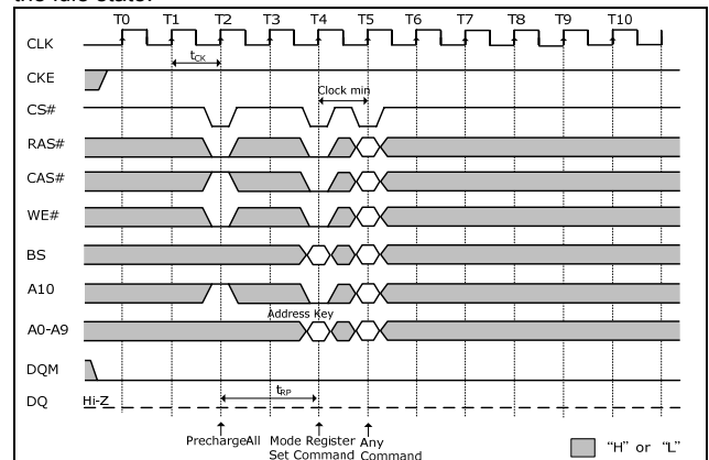
Mode Register Set Cycle (CAS# Latency = 2, 3)
