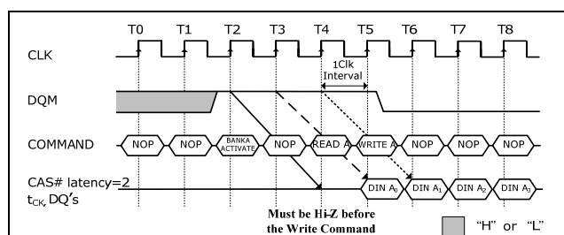
Read to Write Interval (Burst Length \geq 4 , CAS# Latency = 2)
