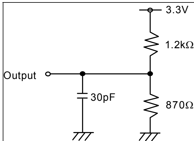
LVTTL D.C. Test Load (A)
