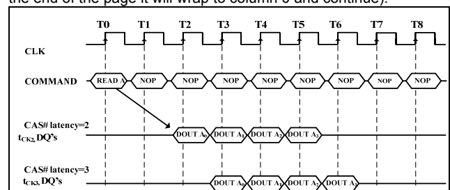
Burst Read Operation (Burst Length = 4, CAS# Latency = 2, 3)
