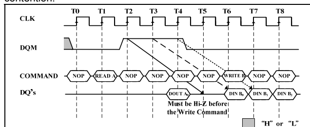
Read to Write Interval (Burst Length \geq 4 , CAS# Latency = 3)
