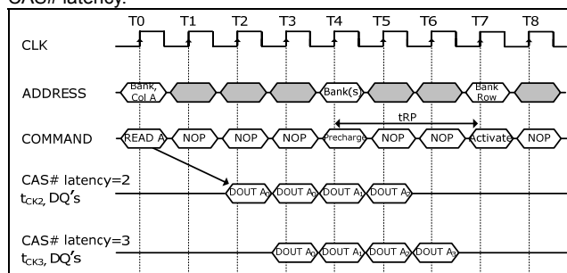
Read to Precharge (CAS# Latency = 2, 3)
