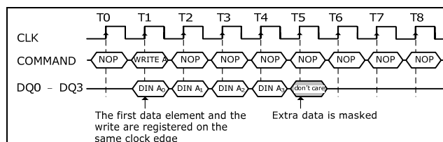
Burst Write Operation (Burst Length = 4, CAS# Latency = 2, 3)
