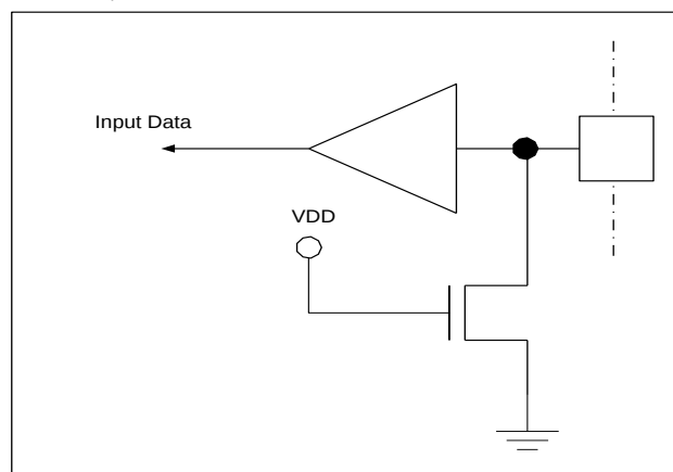
IOEF.0-6: Input Port
