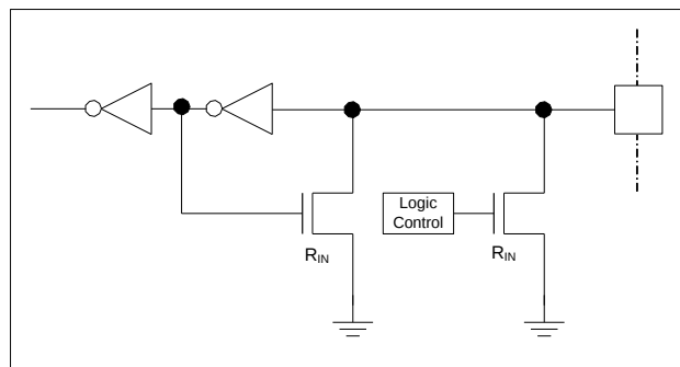
IOEF.0-6: Input Port
