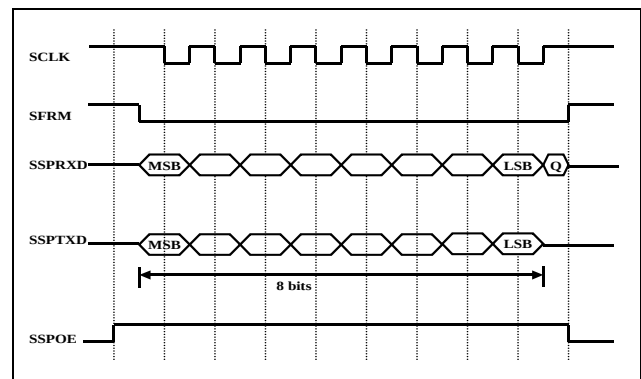
Single transfer Data Change at Rising, Latch at Falling
