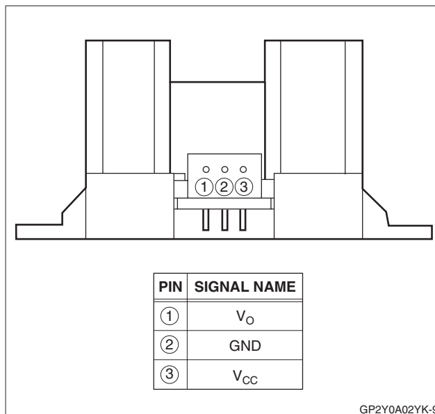
Figure 1. Pinout
