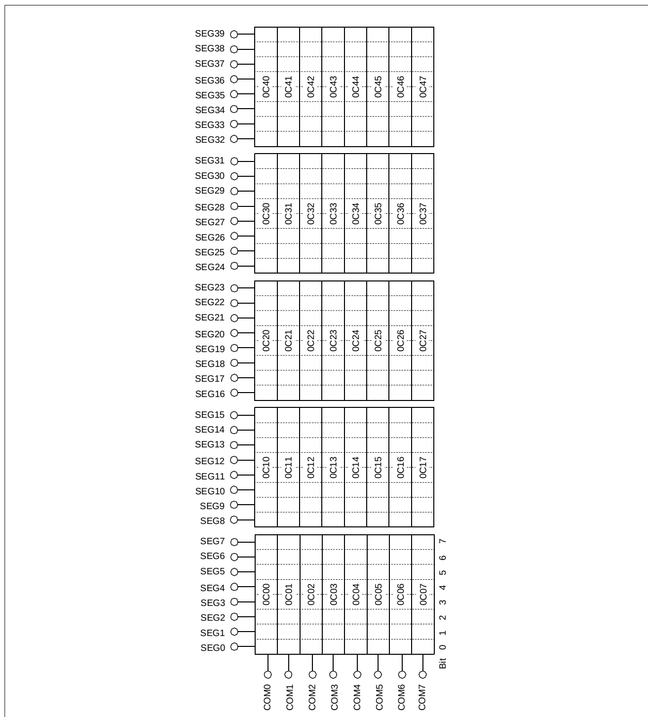
Figure 15-5 LCD Display Memory
