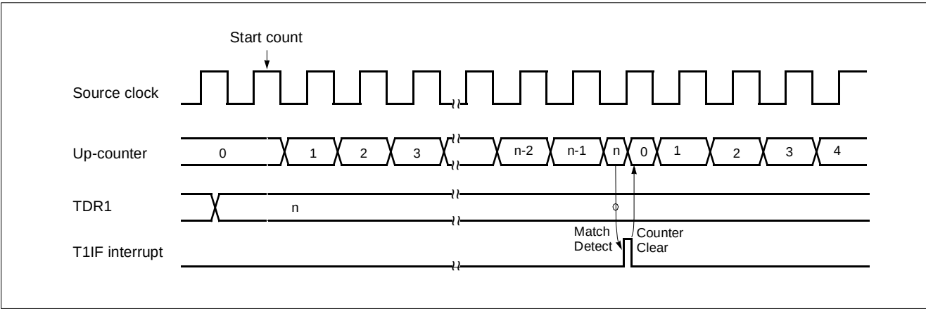
Figure 11-5 Timer Mode Timing Chart
