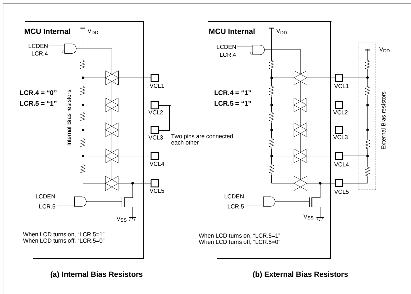
Figure 15-4 Application Example for No Adjusting of Contrast
