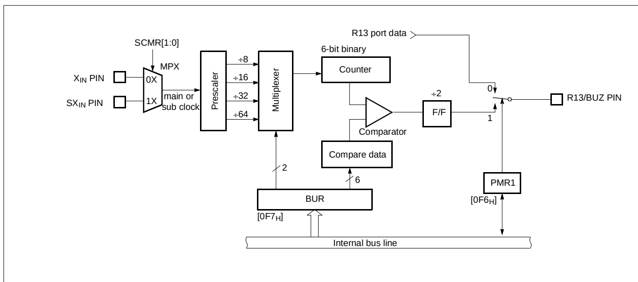
Figure 17-1 Block Diagram of Buzzer Driver
