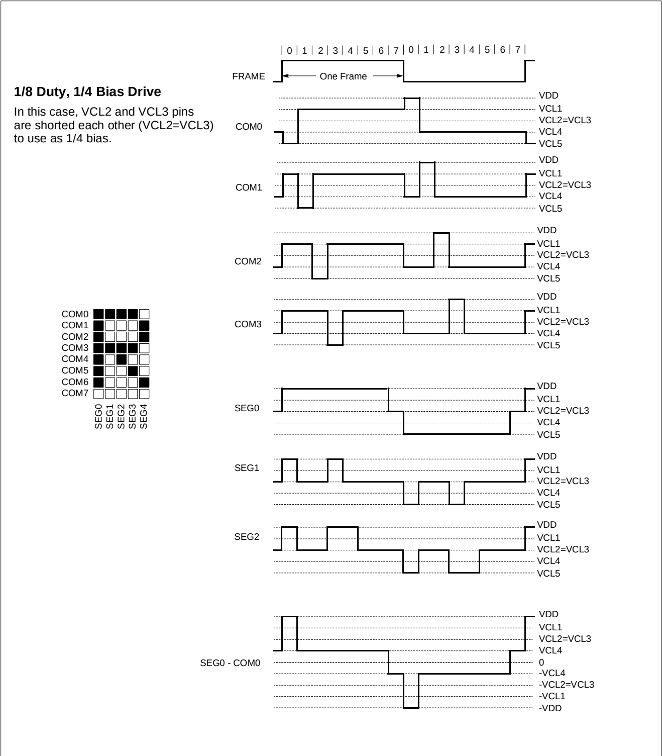
Figure 15-9 Example of LCD drive output
