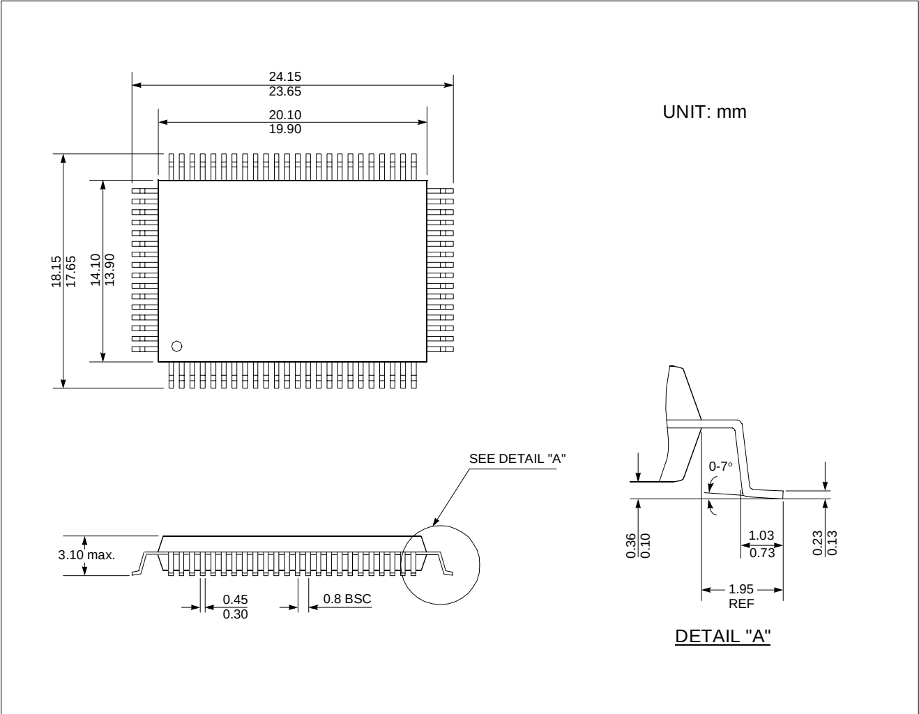
Figure 4-1 Package Diagram
