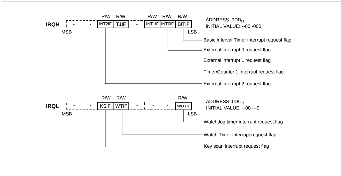
Figure 13-2 Interrupt Request Flag
