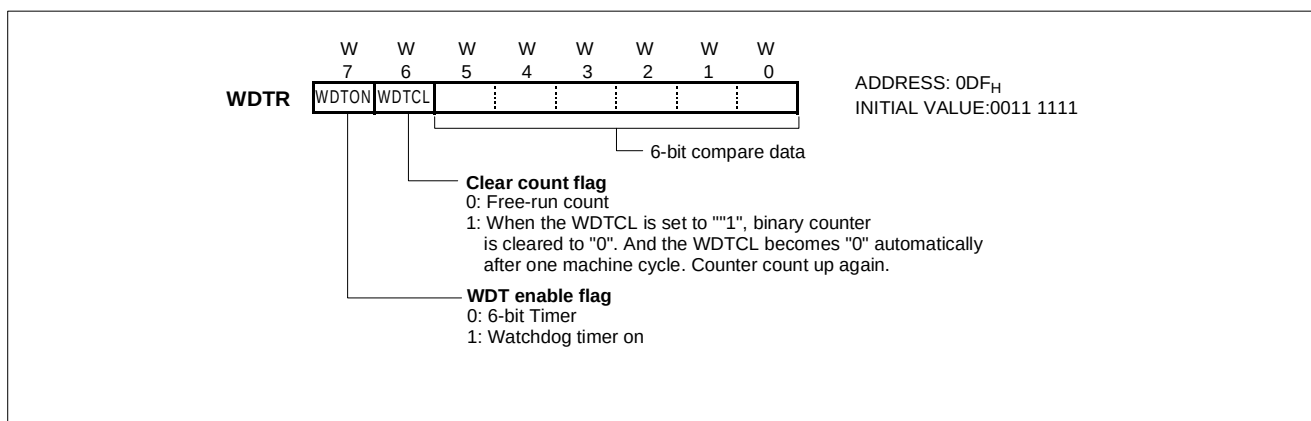
Figure 16-2 WDTR: Watchdog Timer Data Register
