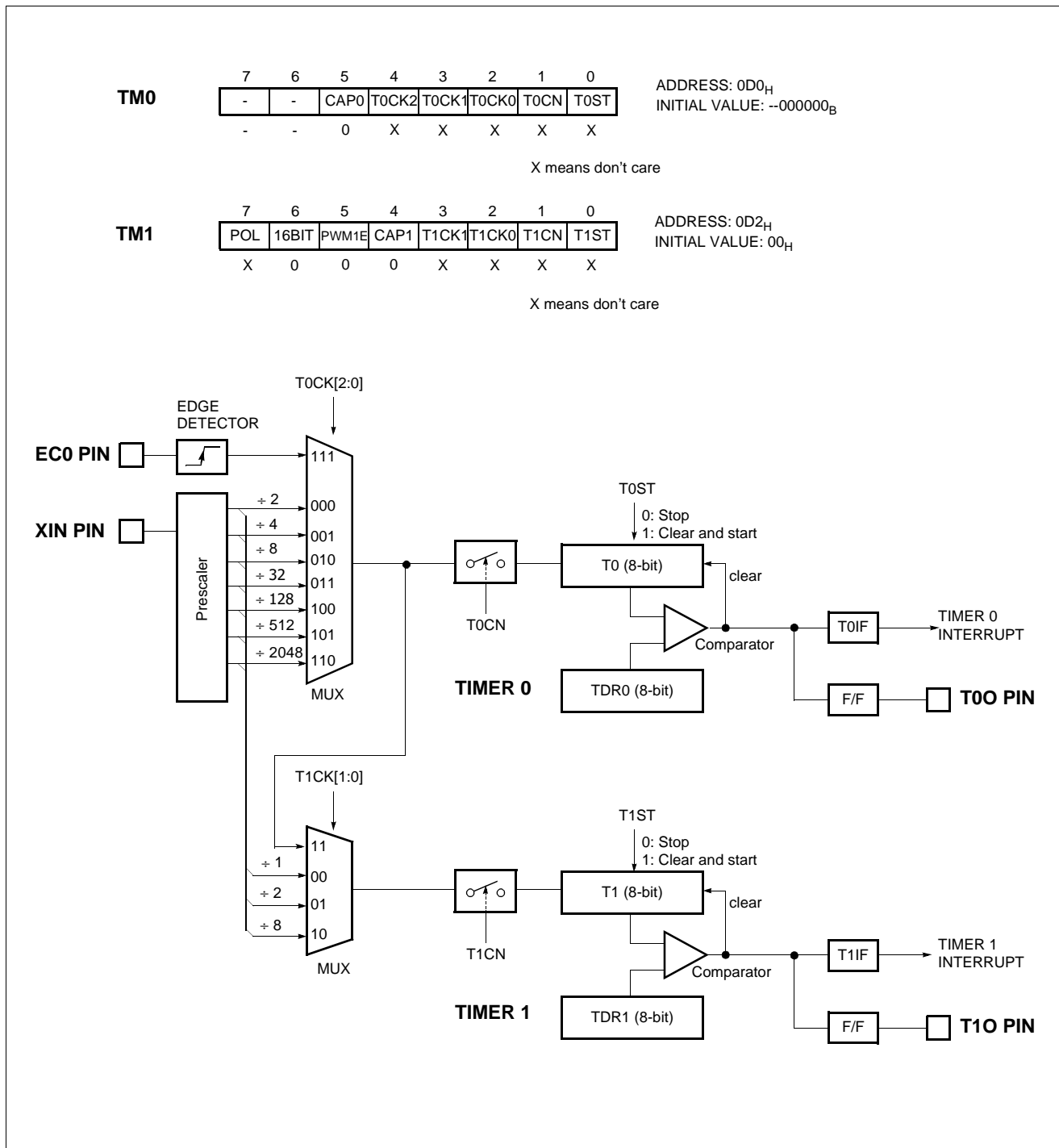
Figure 12-2 8-bit Timer/Counter 0, 1
