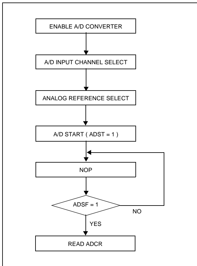
Figure 13-3 A/D Converter Operation Flow
