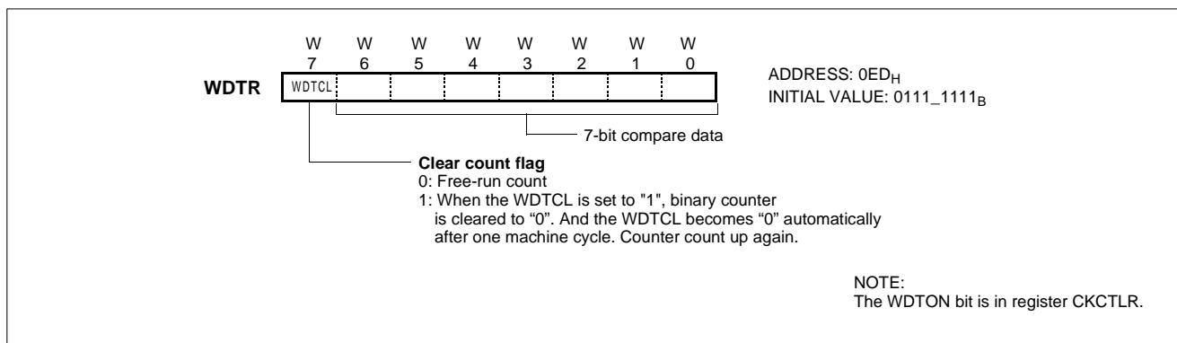
Figure 11-2 WDTDR: Watchdog Timer Data Register
