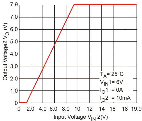
Figure 3. Output Voltage2 vs. Input Voltage
