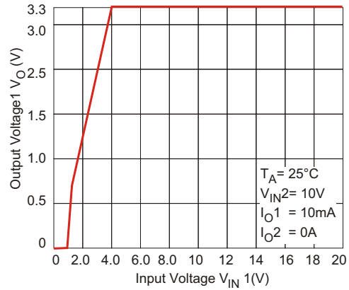
Figure 2. Output Voltage 1 vs. Input Voltage
