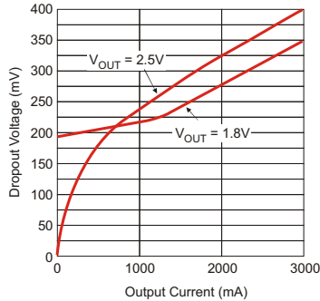
Figure 1. Dropout Voltage vs. Output Current
