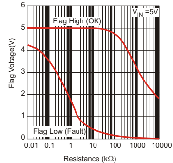
Figure 9. Error Flag Pull-up Resistor
