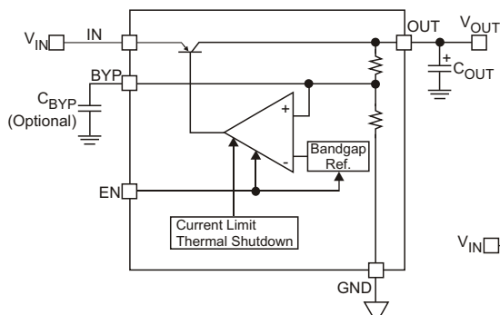
Figure 1. Ultra-Low-Noise Fixed Regulator
