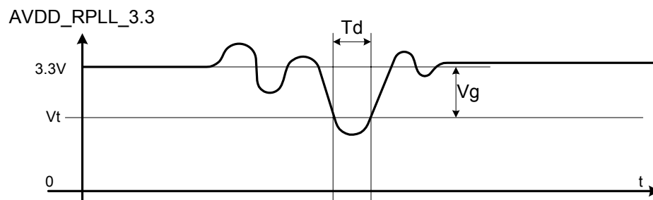
Figure 7: Reset Power Supply Glitch
