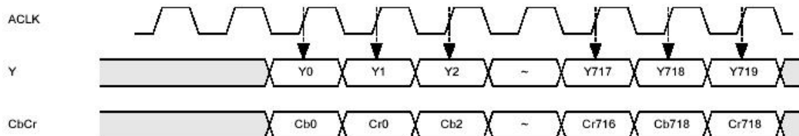
Figure 16: 16-bit 4:2:2 YCbCr/YPbPr
