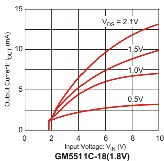
(7) P-ch DRIVER OUTPUT CURRENT VS. INPUT VOLTAGE
