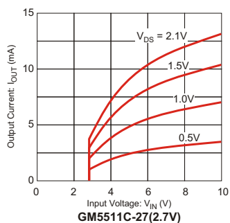
(7) P-ch DRIVER OUTPUT CURRENT VS. INPUT VOLTAGE
