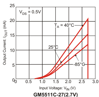
(6) N-ch DRIVER OUTPUT CURRENT VS. INPUT VOLTAGE
