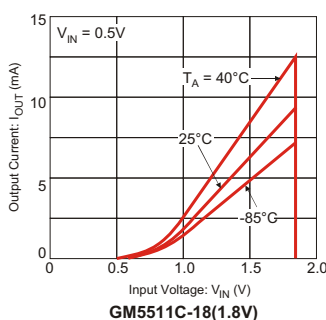
(6) N-ch DRIVER OUTPUT CURRENT VS. INPUT VOLTAGE
