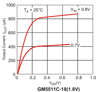
(4) N-ch Driver Output current vs. V_{DS}
