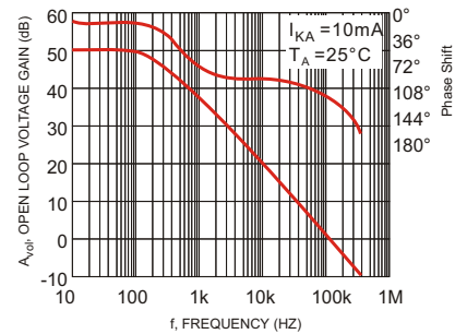
Figure 14. Open-Loop Voltage Gain vs. Frequency
