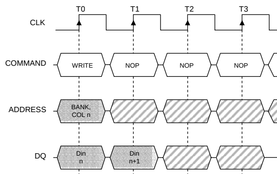
Figure 14. WRITE Burst
