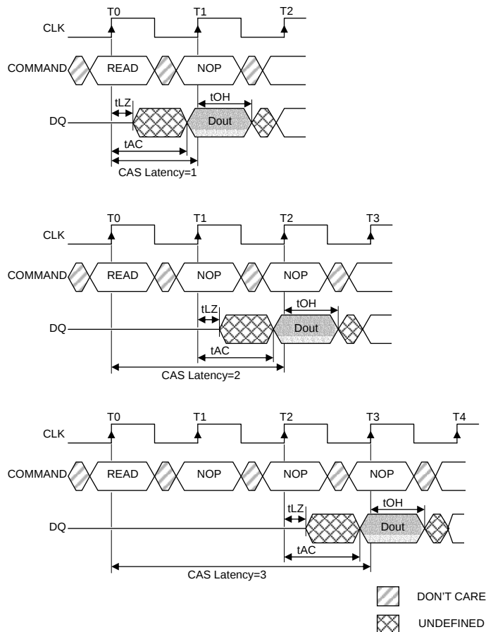
Figure 6. CAS Latency
