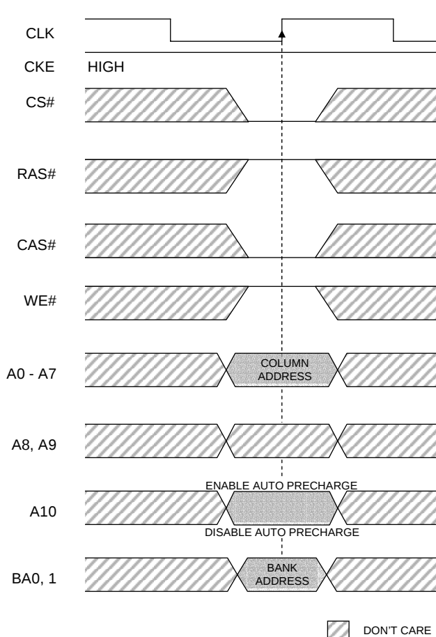
Figure 5. READ Command
