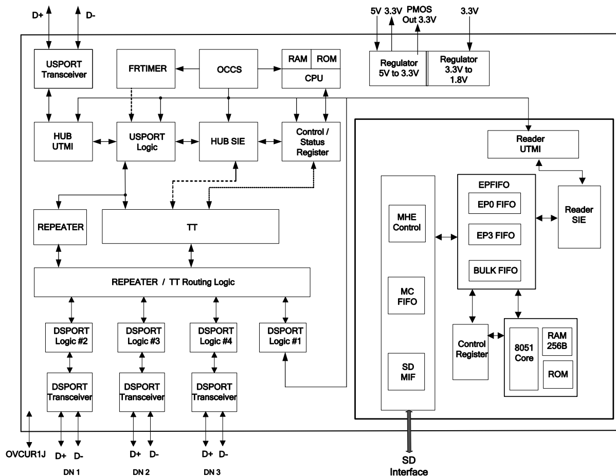
Figure 4.1- GL857L Block Diagram
