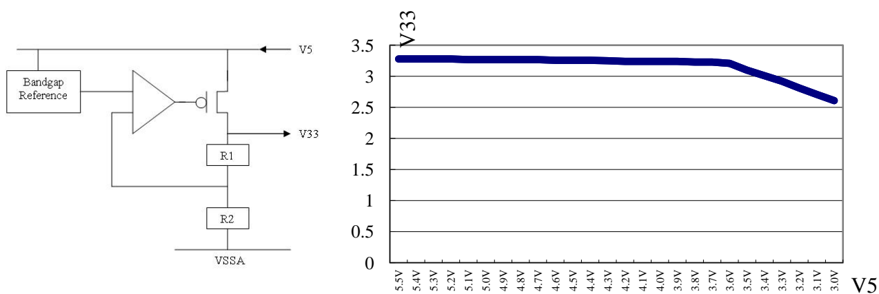
Figure 6.1 - V_{in}(V5) vs V_{out}(V33) *
