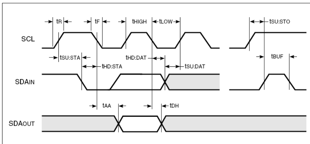
Bus Timing
