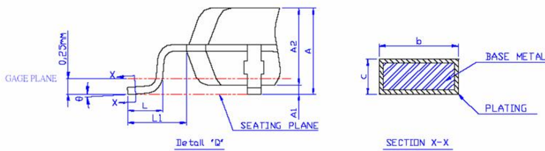
Figure 8.2- GL843 208 Pin QFP Package
