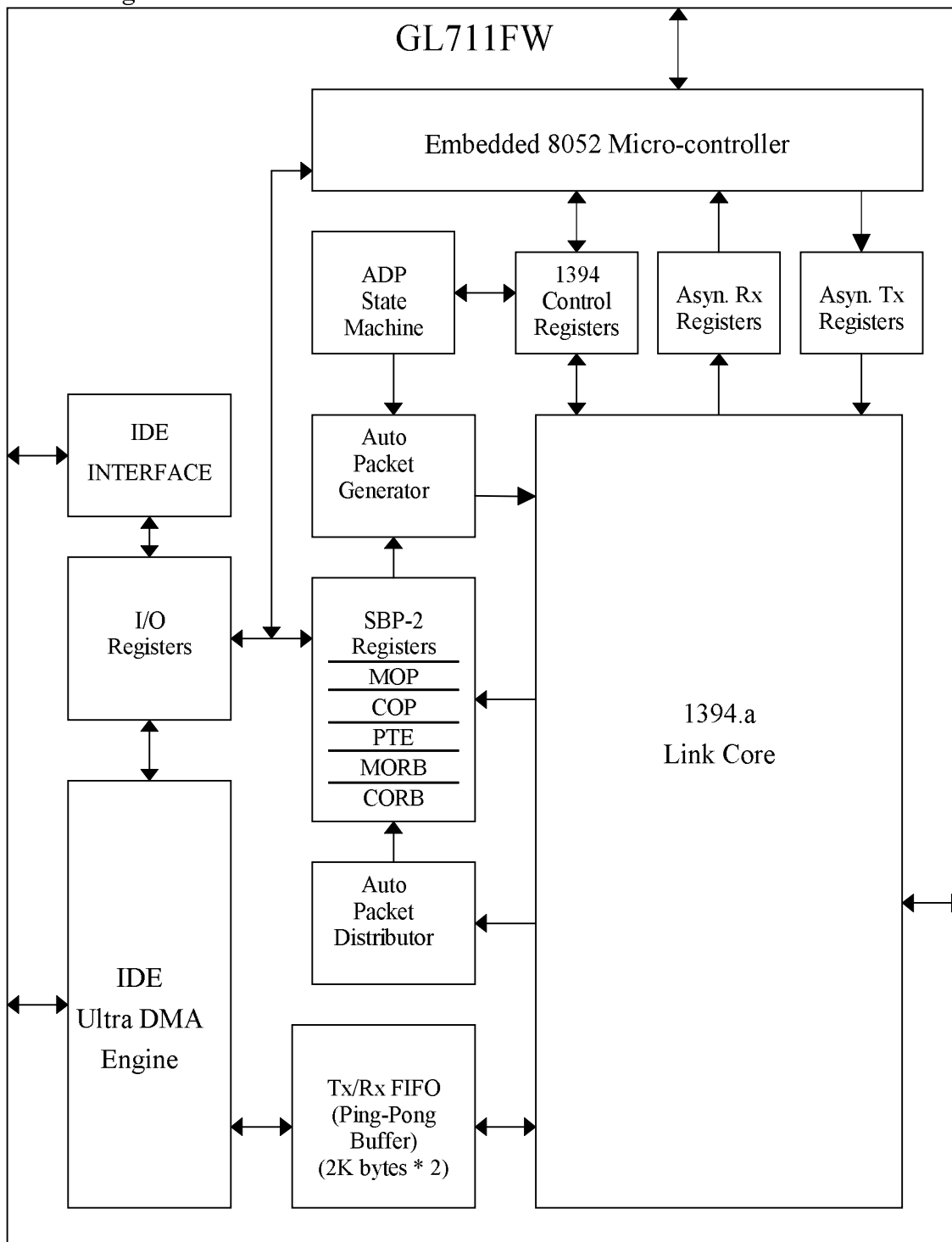
Block Diagram
