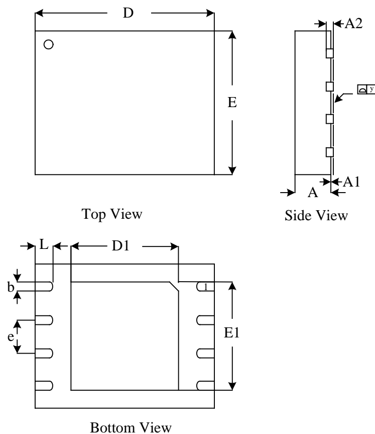
Figure29. WSON8 (8*6mm)
