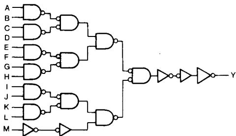
Fig. 1 Logic diagram
