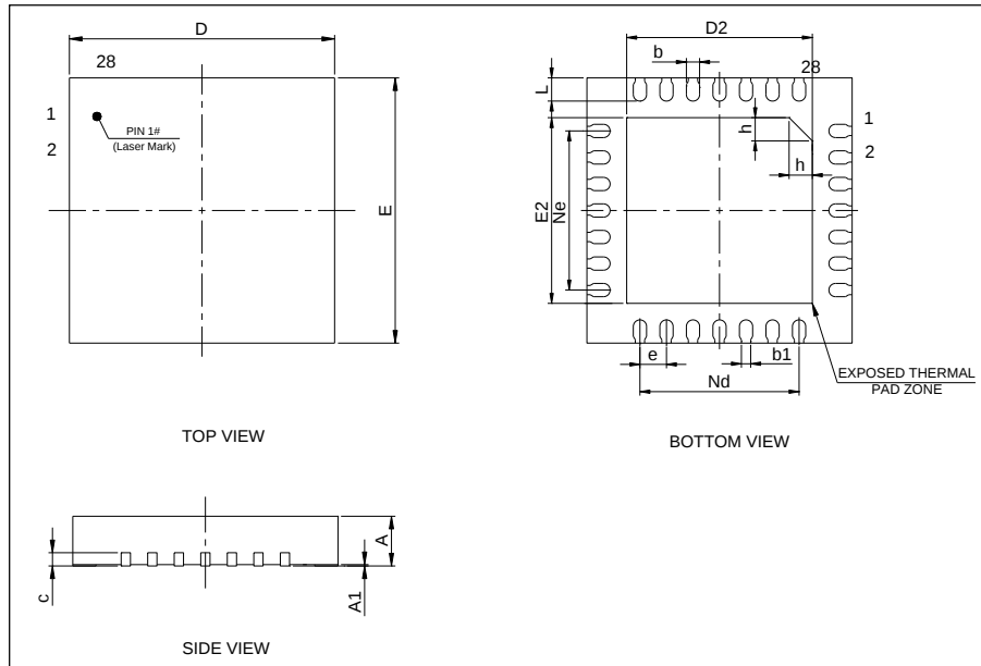
Figure 5-9. QFN28 package outline
