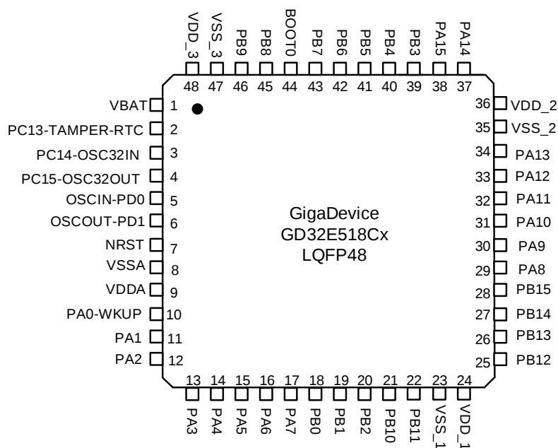
Figure 2-5. GD32E518Cx LQFP48 pinouts
