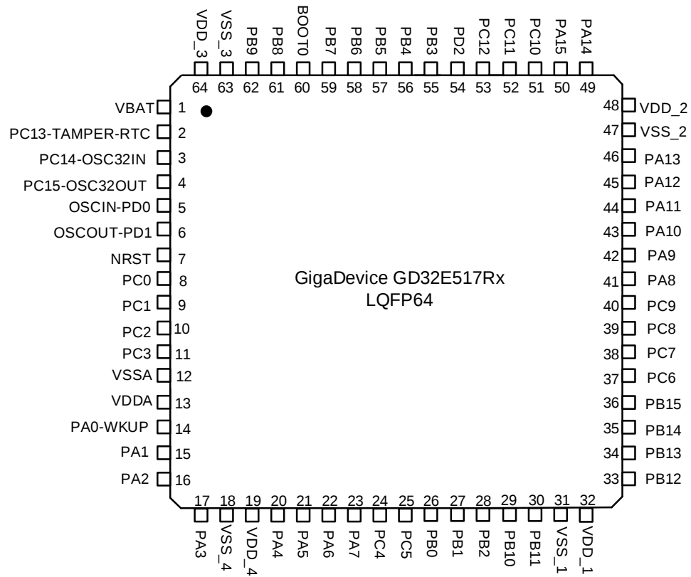
Figure 2-4. GD32E517Rx LQFP64 pinouts
