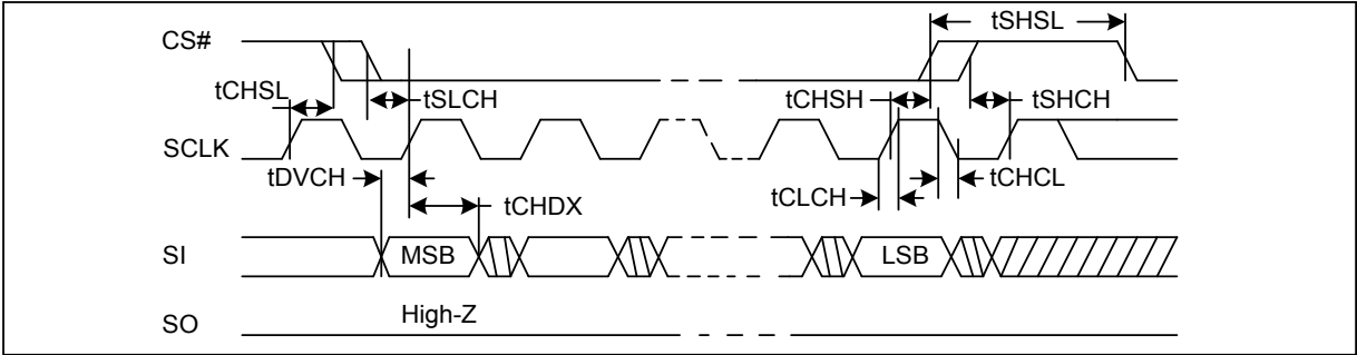
Figure41. Serial Input Timing Diagram
