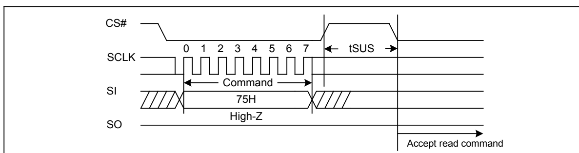
Figure 31. Program/Erase Suspend Sequence Diagram
