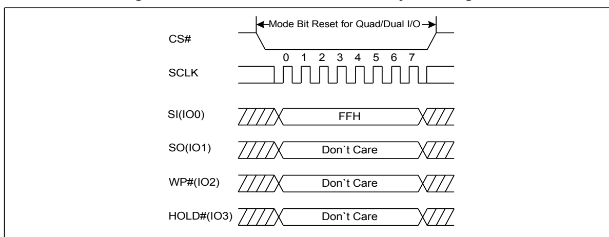
Figure 30. Continuous Read Mode Reset Sequence Diagram
