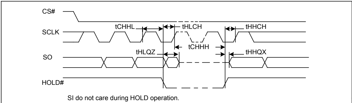
Figure 42. Hold Timing
