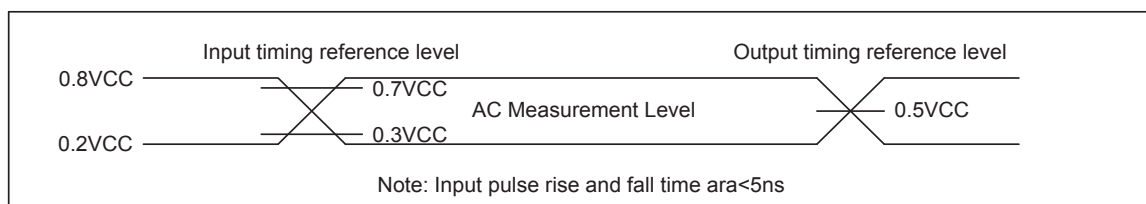
Figure 39. Input Test Waveform and Measurement Level
