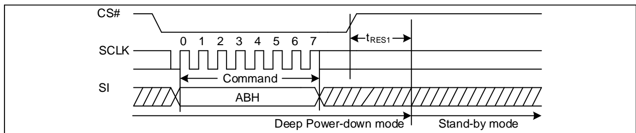
Figure26. Release Power-Down/Read Device ID Sequence Diagram
