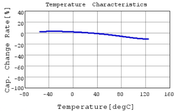
GCM033R71A472KA03 C-Temp. capchange, DC0.0V,
