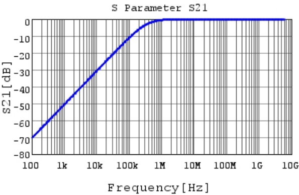
GCM033R71A472KA03 S21 DC0V, 25degC
