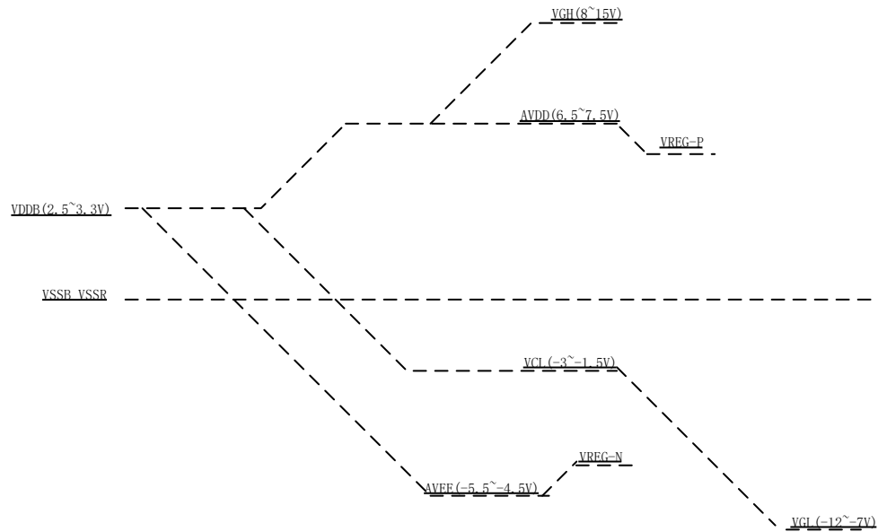
LCD power generation scheme
