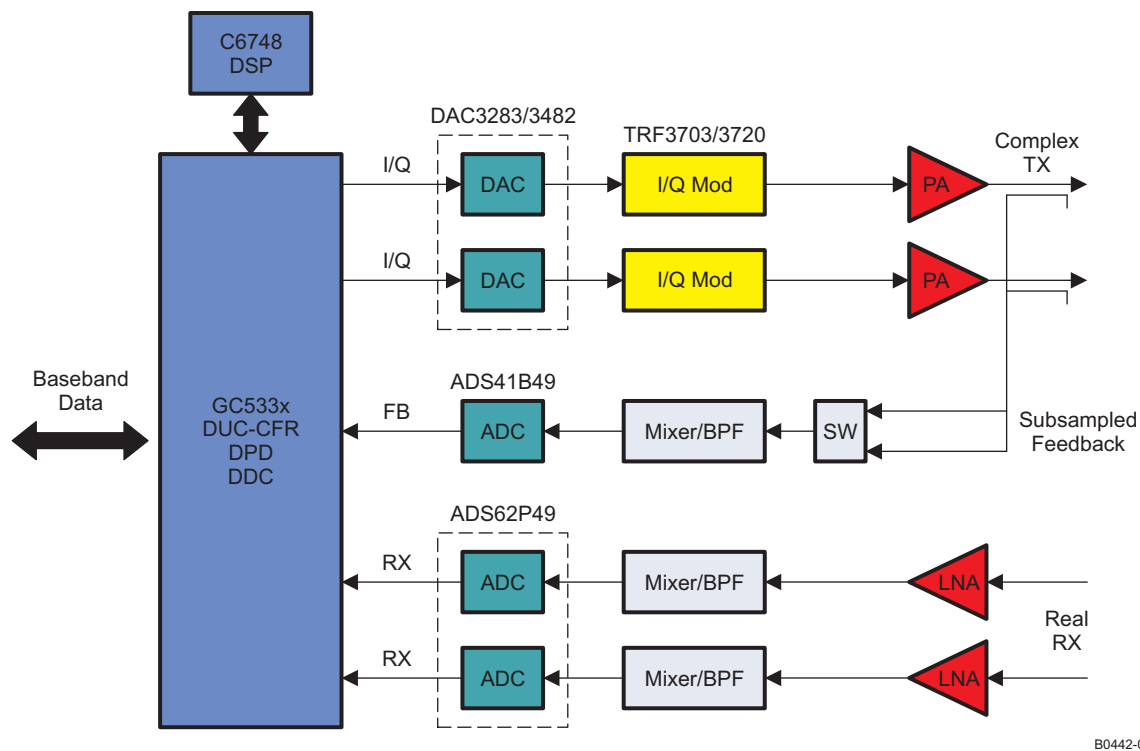
Figure 1. Two-Antenna-Mode Subsampled-Feedback Diagram
