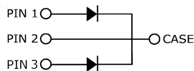
TO-247-3 Package
