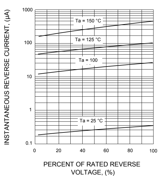
FIG.4 - TYPICAL REVERSE CHARACTERISTICS PER DIODE
