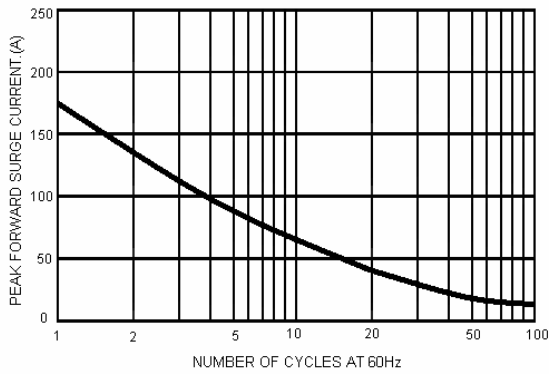
FIG.1-MAXIMUM NONO-REPETITIVE FORWARD SURGE CURRENT PER BRIDGE ELELMENT
