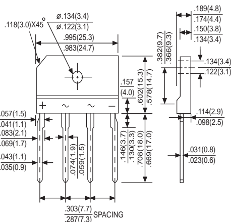
GBJ4-10
